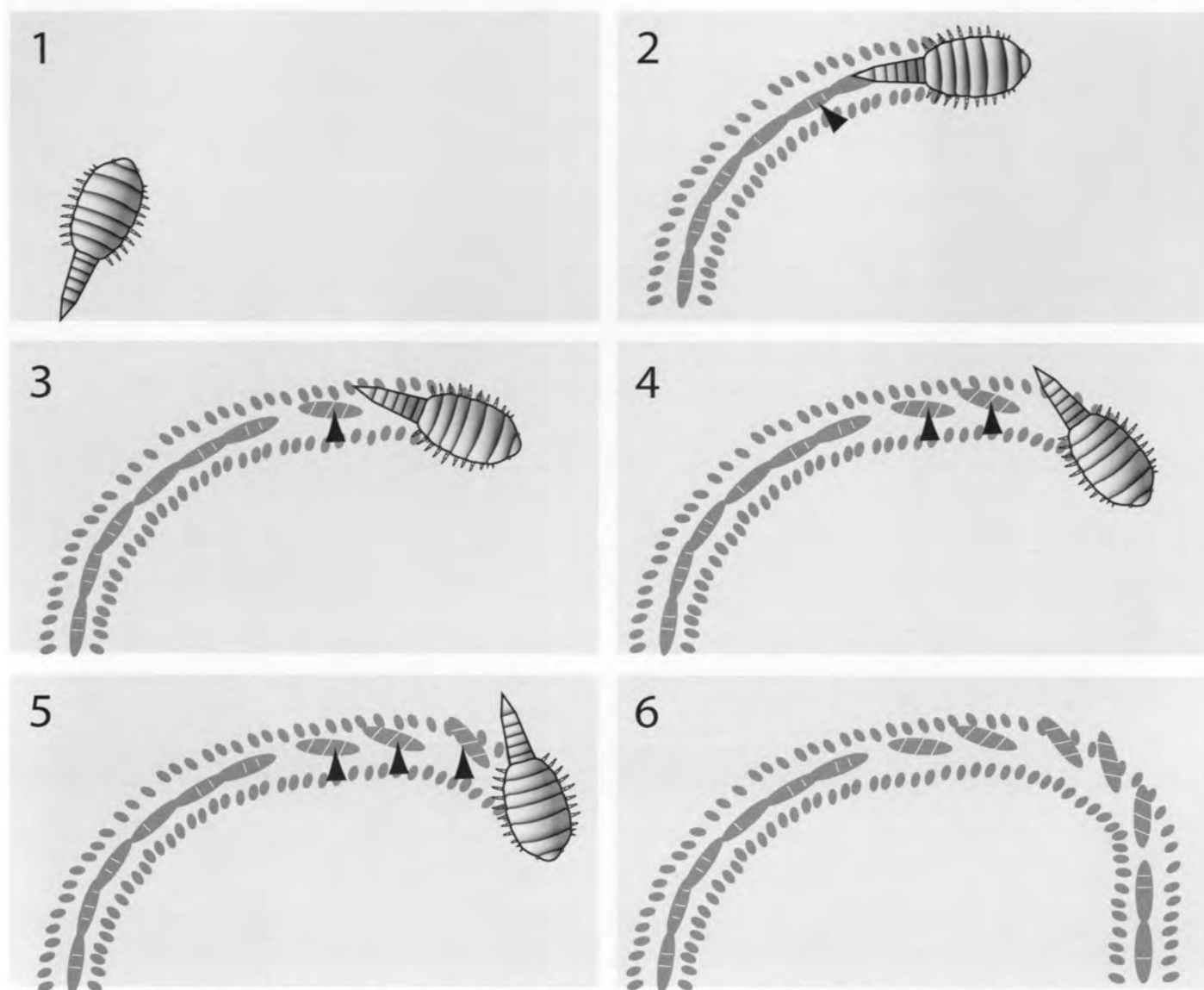
FIGURE 3—Hypothetical model of Protichnites eremita Form 2 production by the euthycarcinoid arthropod Mosinea macnaughtoni . 1, euthycarcinoid travelling in an arcuate pathway; 2, continuing on arcuate path, impressions produced by the animal's postabdomen are confined to the medial portion of the trackway (arrowhead); 3–5, continued forward motion, combined with an increasing turn radius, pulse-like locomotion, and little to no lateral flexibility in the postabdomen of the producer begin to produce outward-swinging postabdominal imprints (arrowed), such as those observed in Trackway B (Fig. 1); 6, turn completed, the producer resumes a straight path.
