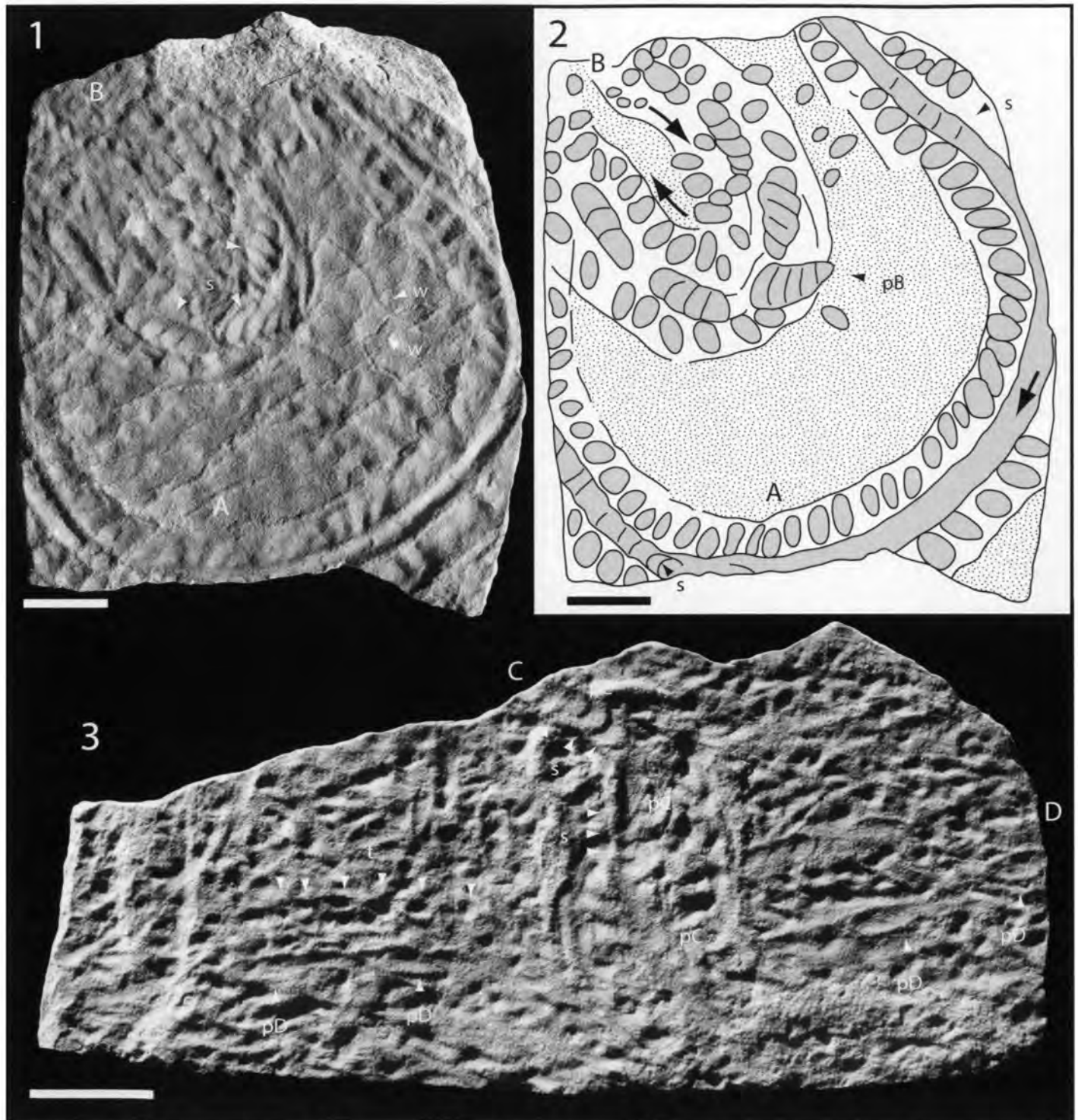
FIGURE 1— Protichnites eremita Form 2, Trackways A and B, Elk Mound Group, Blackberry Hill, Wisconsin, PRI Station 3421. 1, PRI 10143, both trackways shown, Trackway B exhibits a sharp right turn whereas Trackway A exhibits a gentle turn; segmentation present in the intermittent medial impressions (Fig. 1.1, arrowed s; Fig. 1.2) is well-defined, as is the microbially mediated wrinkle texture (arrowed w); 2, line drawing of PRI 10143 showing morphology of trackways A and B in Figure 1.1; segmented intermittent medial impressions (arrowed p), interpreted as representing impressions of an apodous postabdomen of at least five somites; arrows point in the direction of travel; tracks and imprints of Trackways A and B are shaded gray for clarity; 3, PRI 11040, Protichnites eremita Form 2, Trackways C and D. Abbreviations: p=postabdominal imprint, s=segment, t=track. Photos lit from top-left. Scale bars=4 cm.
