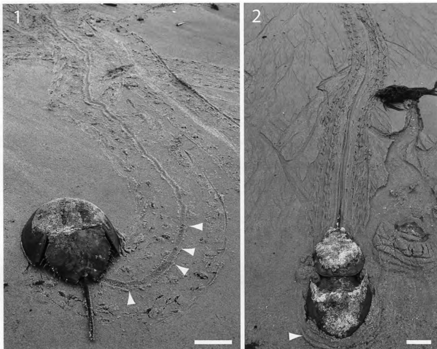
FIGURE 4— Limulus polyphemus . 1, solitary animal and its trackway after making a sharp turn, the medial drag made by its telson exhibits weak segmentation (arrowheads); 2, pair in amplexus showing a combined trackway, note sediment accumulation at the anterior of the female's carapace (arrowhead) that has been 'plowed' forward by the motion of the paired animals. Scale bar=10 cm. Images from G. Gauvry.
